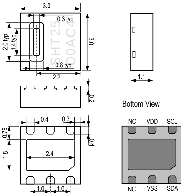
Figure 1: Drawing of SHT25 sensor package, dimensions are given in mm (1mm = 0.039inch), tolerances are \pm 0.1 mm. The die pad (center pad) is internally connected to VSS. The NC pads must be left floating. VSS = GND, SDA = DATA. Numbering of E/O pads starts at lower right corner (indicated by notch in die pad) and goes clockwise (compare Table 2).
