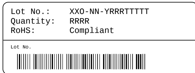
Figure 20: First label on reel: XX = Sensor Type (25 for SHT25), O = Output mode (0 = Digital), NN = Chip Version, Y = last digit of year, RRR = number of sensors on reel divided by 10 (200 for 2000 units), TTTTT = Traceability Code.
