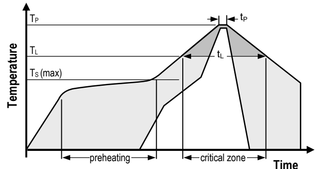
Figure 9 Soldering profile according to JEDEC standard. T_P \leq 260^\circ\text{C} and t_P < 40\text{sec} for Pb-free assembly. T_L < 220^\circ\text{C} and t_L < 150\text{sec} . Ramp-up/down speeds shall be < 5^\circ\text{C}/\text{sec} .
