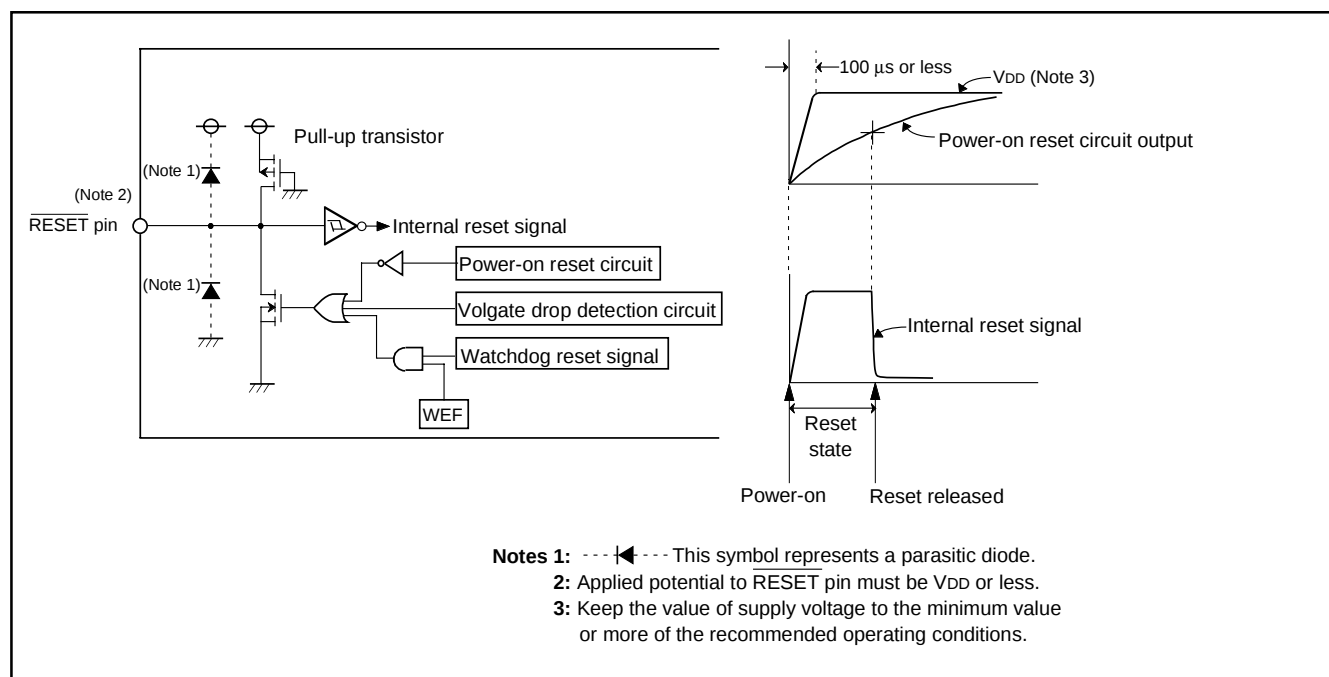
Fig. 35 Structure of reset pin and its peripherals, and power-on reset operation
