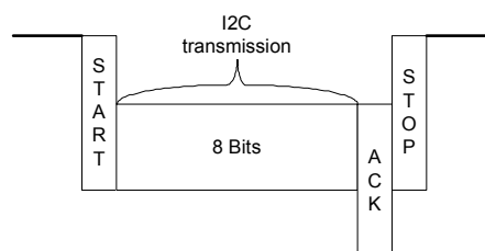
Figure 20: I 2 C communication
