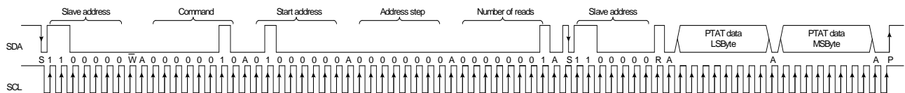
Figure 9 PTAT (SA = 0x60, command = 0x02, Start address = 0x40, Address step = 0x00, Number of reads = 0x01) measurement result read
