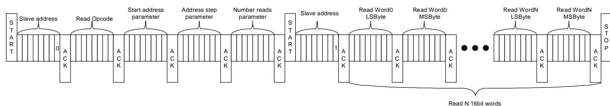
Figure 23: RAM readout command structure
