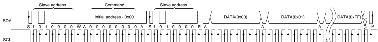
Figure 4 Whole EEPROM dump (SA = 0x50, command = 0x00)
