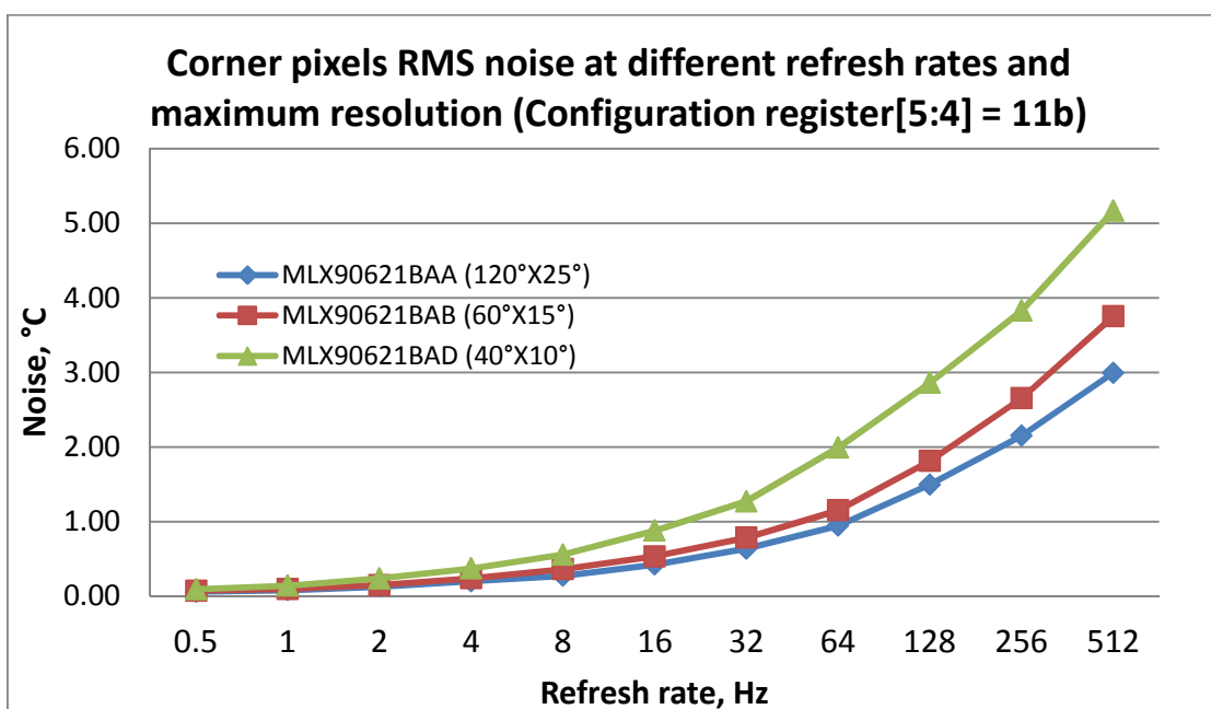
Figure 28: Corner pixels noise
