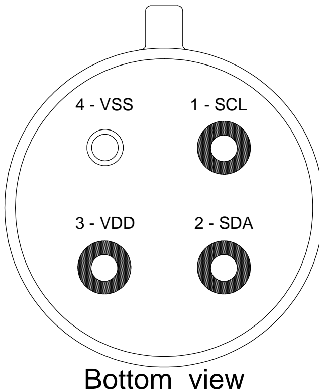
Figure 1 Pin description
