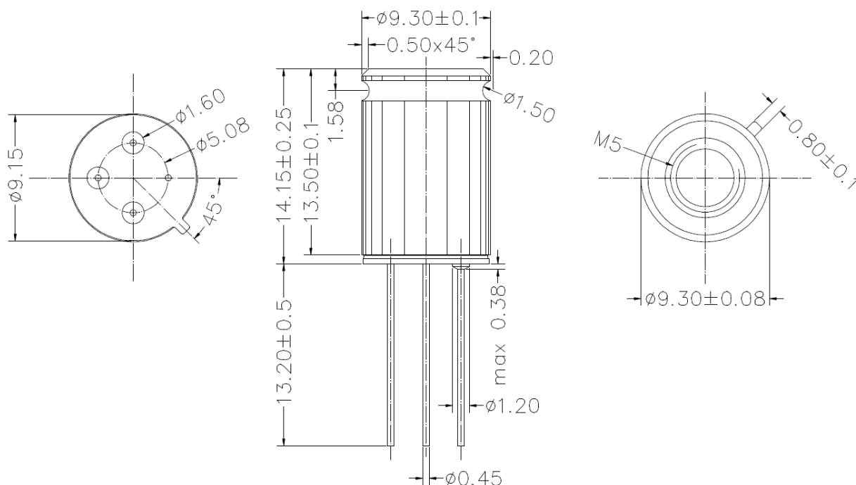
Figure 33 Mechanical drawing of Medium (40x10) FOV device (MLX90621BAD)
