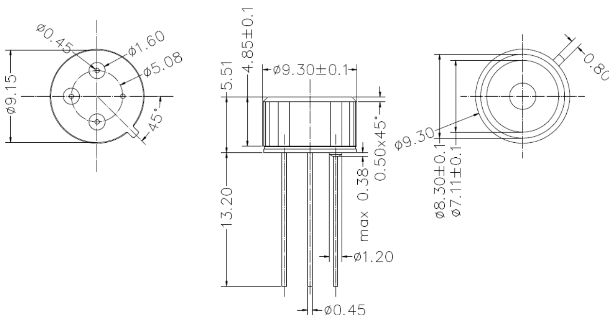
Figure 31 Mechanical drawing of Wide (120x25) FOV device (MLX90621BAA)
