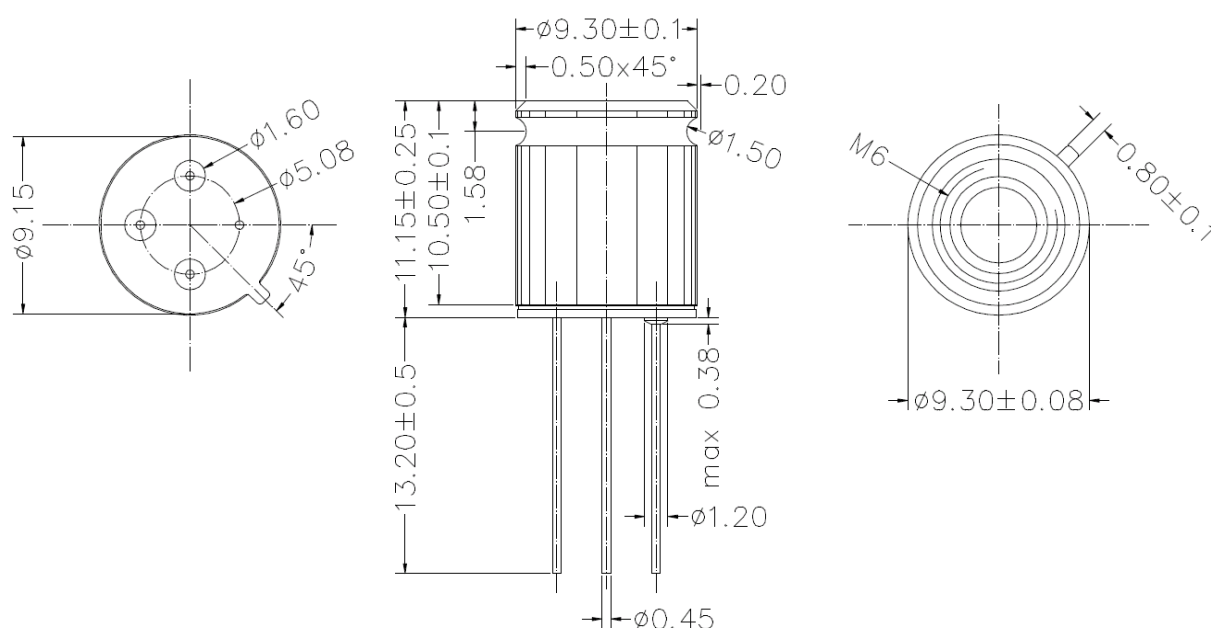
Figure 32 Mechanical drawing of Wide (60x16) FOV device (MLX90621BAB)
