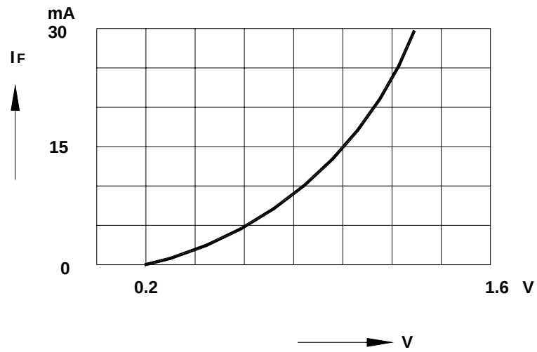
Forward Characteristics
