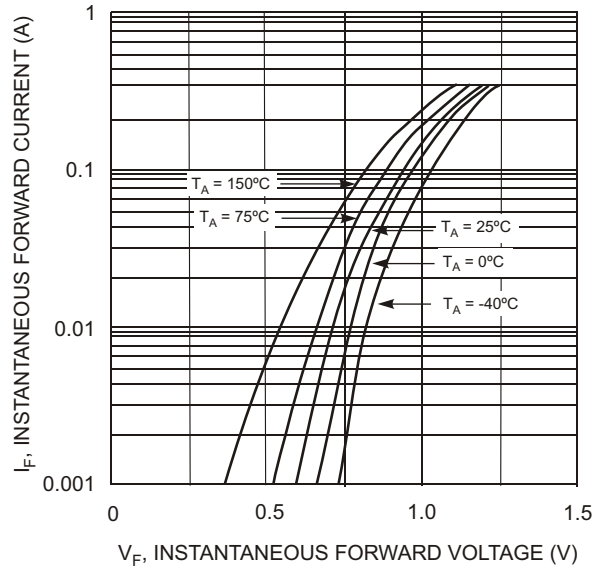
Fig. 2 Forward Characteristics
