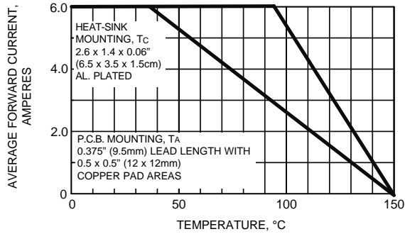
FIG. 1 - DERATING CURVE OUTPUT RECTIFIED CURRENT
