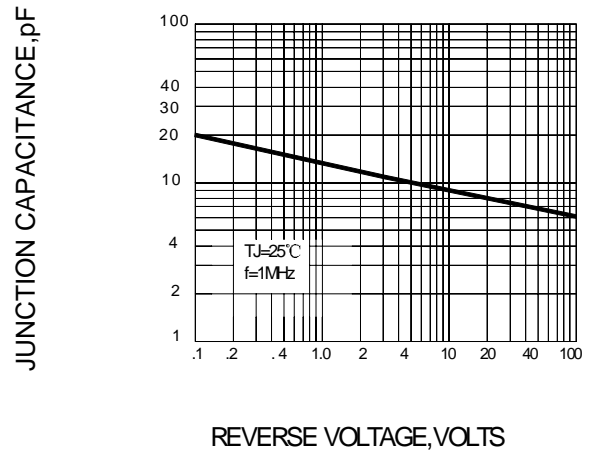
FIG.4–PEAK JUNCTION CAPACITANCE
