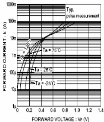
Fig. 1 Forward characteristics
