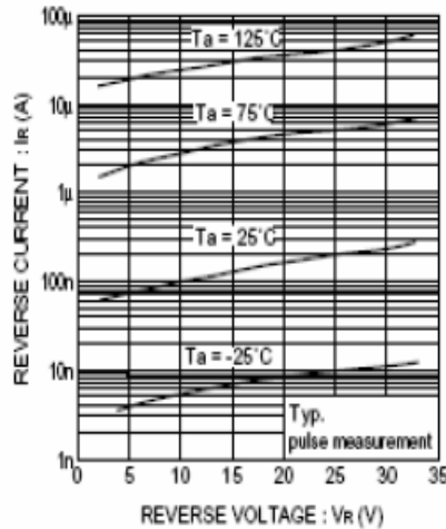
Fig. 2 Reverse characteristics
