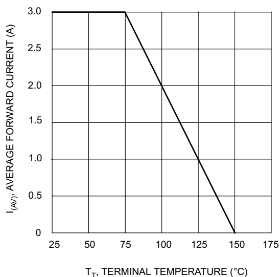
T_T , TERMINAL TEMPERATURE ( ^{\circ}\text{C} ) Fig. 1 Forward Current Derating Curve
