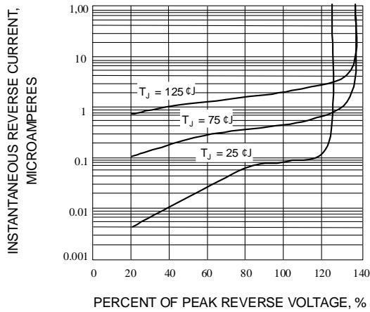
Fig. 3-TYPICAL REVERSE CHARACTERISTICS
