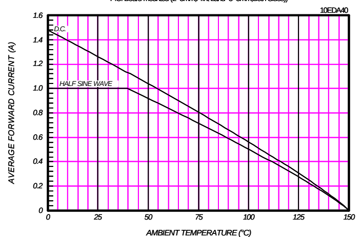
AVERAGE FORWARD CURRENT VS. AMBIENT TEMPERATURE
