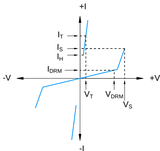
Figure1 - V-I Characteristics
