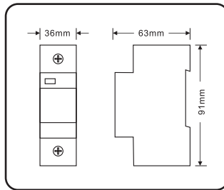
TA100B 尺寸图 TA100B Dimension diagram
