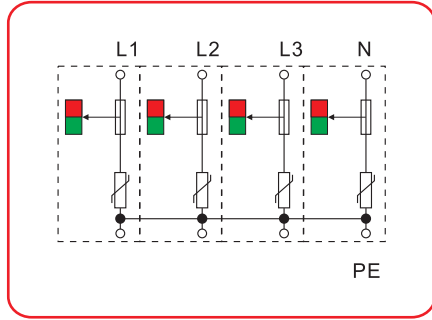
TA100B 基本电路图 TA100B Basic circuit diagram
